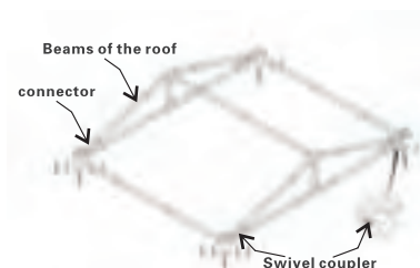
6.Connect the peaked roof
